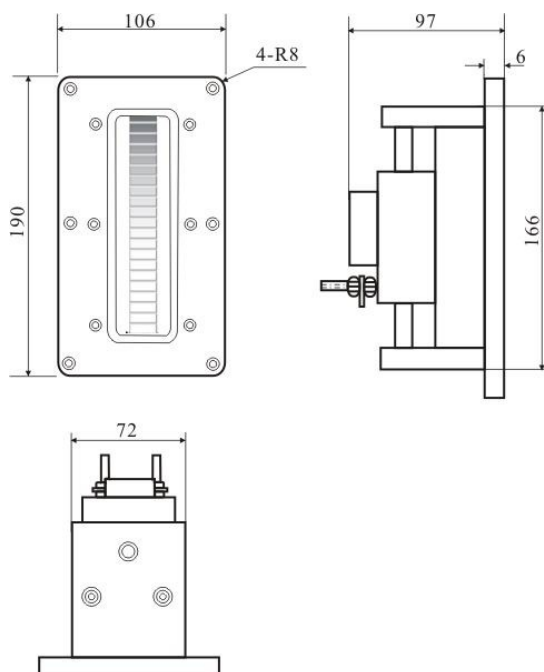
G1 mounting drawing
